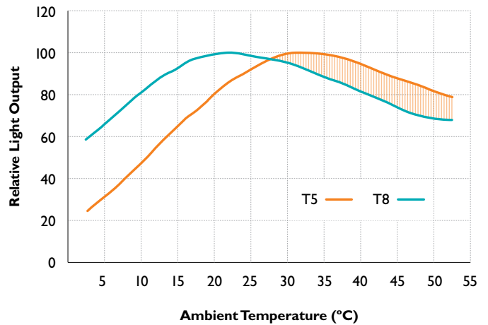
Relative Light Output vs. Ambient Temperature
